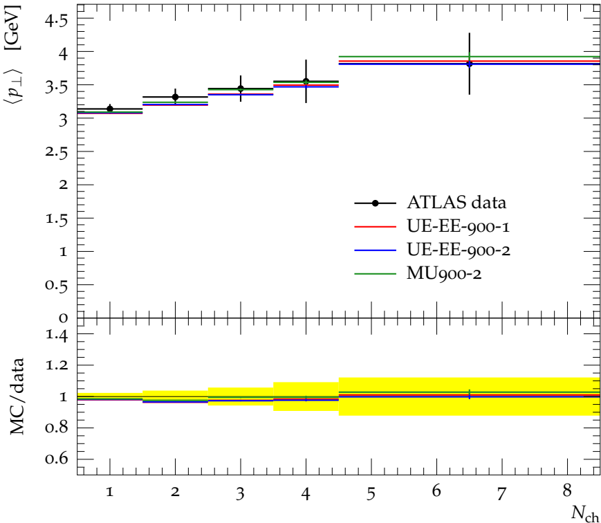
Charged \langle p_{\perp} \rangle vs. N_{\text{ch}} at 900 GeV, track p_{\perp} > 2500 MeV, for N_{\text{ch}} \geq
