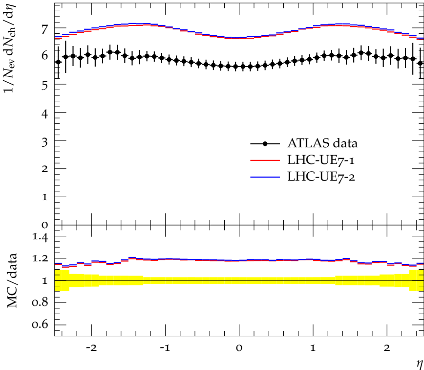
Charged particle \eta at 7 TeV, track p_{\perp} > 100 MeV, for N_{\text{ch}} \geq 2
