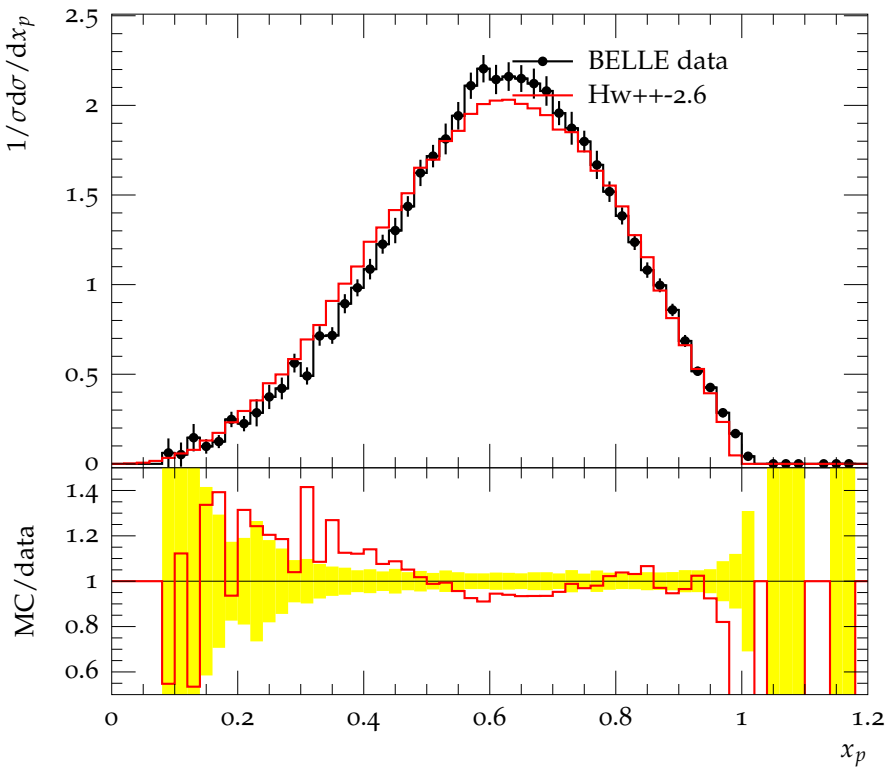
D^{*+} \rightarrow D^0 \pi^+ scaled momentum in the continuum region
