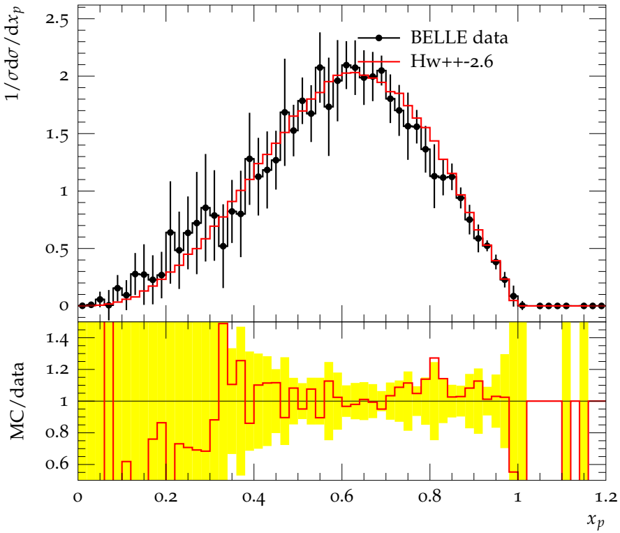
D^{*+} \rightarrow D^+ \pi^0 scaled momentum in the continuum region
