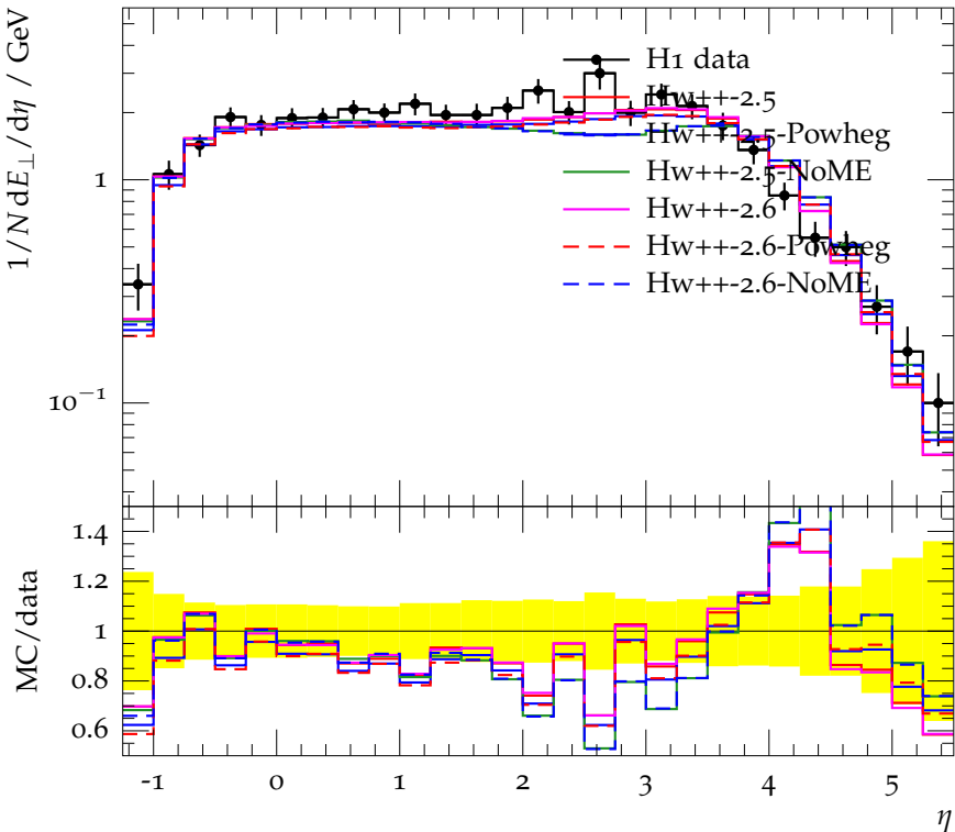
Transverse energy flow as a function of rapidity, x < 10^{-3}
