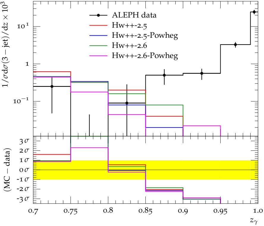
Photon Fragmentation in 3-jet events with y_{\text{cut}} = 0.1
