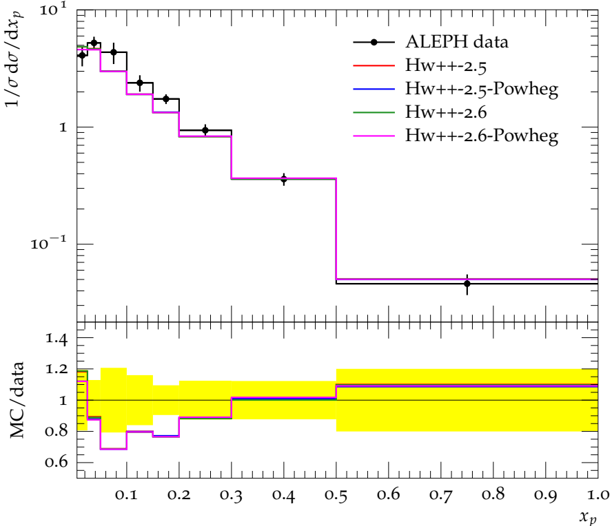
K^{*0}(892) spectrum
