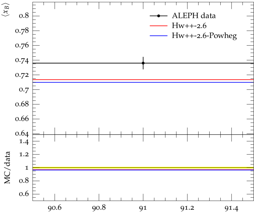
Mean of b quark fragmentation function f(x_B^{\text{lead}})
