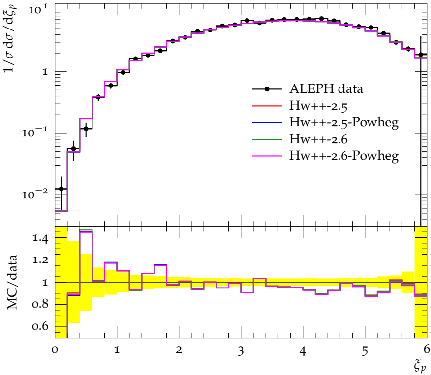
Charged particle spectrum ( E_{\text{CMS}} = 133 \text{ GeV} )
