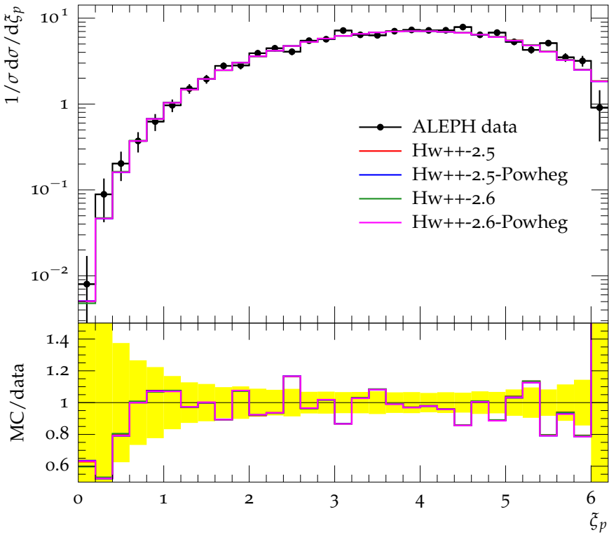
Charged particle spectrum ( E_{\text{CMS}} = 172 \text{ GeV} )
