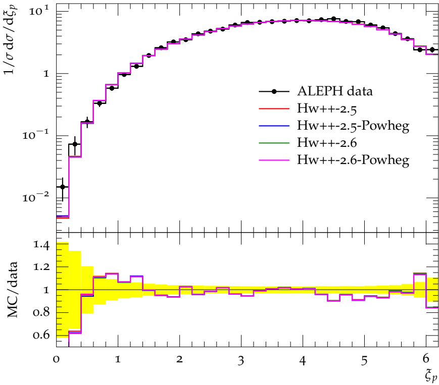
Charged particle spectrum ( E_{\text{CMS}} = 183 \text{ GeV} )
