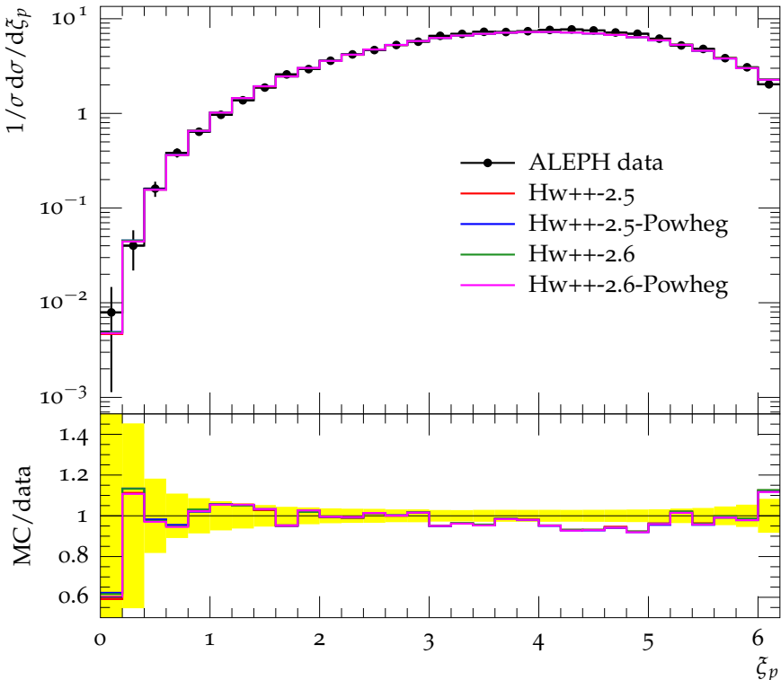
Charged particle spectrum ( E_{\text{CMS}} = 196 \text{ GeV} )
