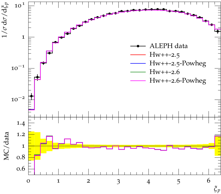
Charged particle spectrum ( E_{\text{CMS}} = 206 \text{ GeV} )
