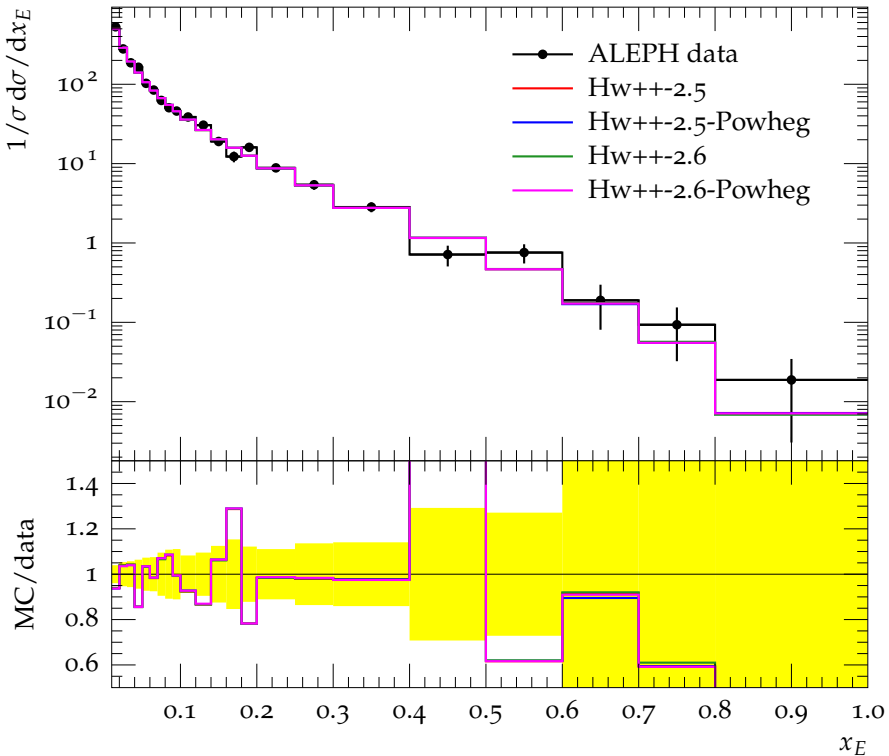
Charged particle spectrum ( E_{\text{CMS}} = 172 \text{ GeV} )
