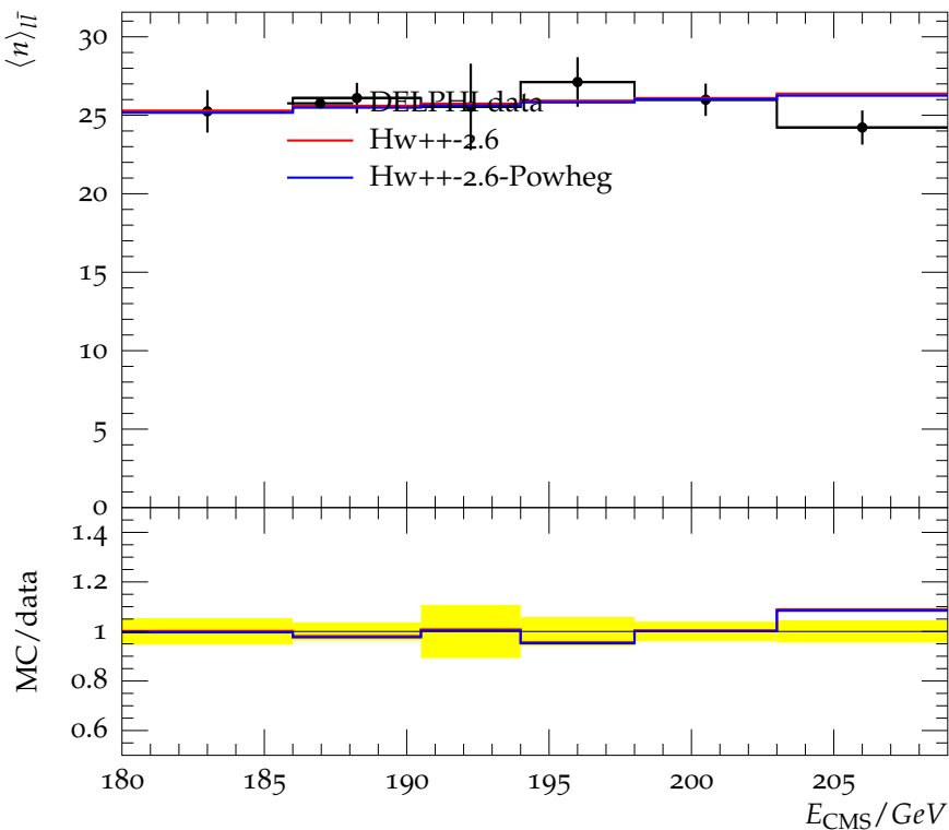
Charged multiplicity as a function of energy in uds events
