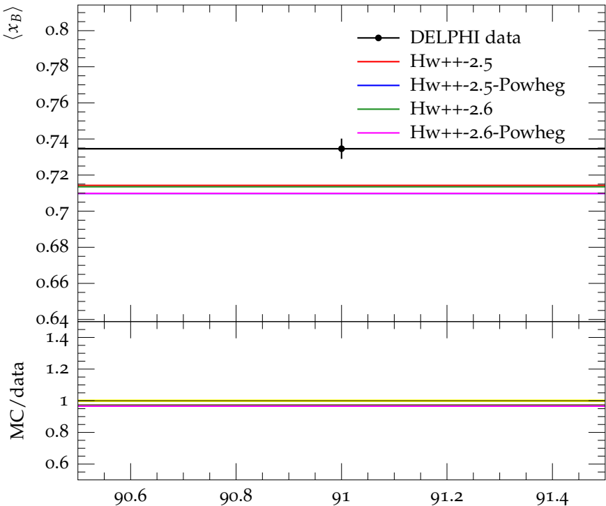
Mean of b quark fragmentation function f(x_B^{\text{prim}})
