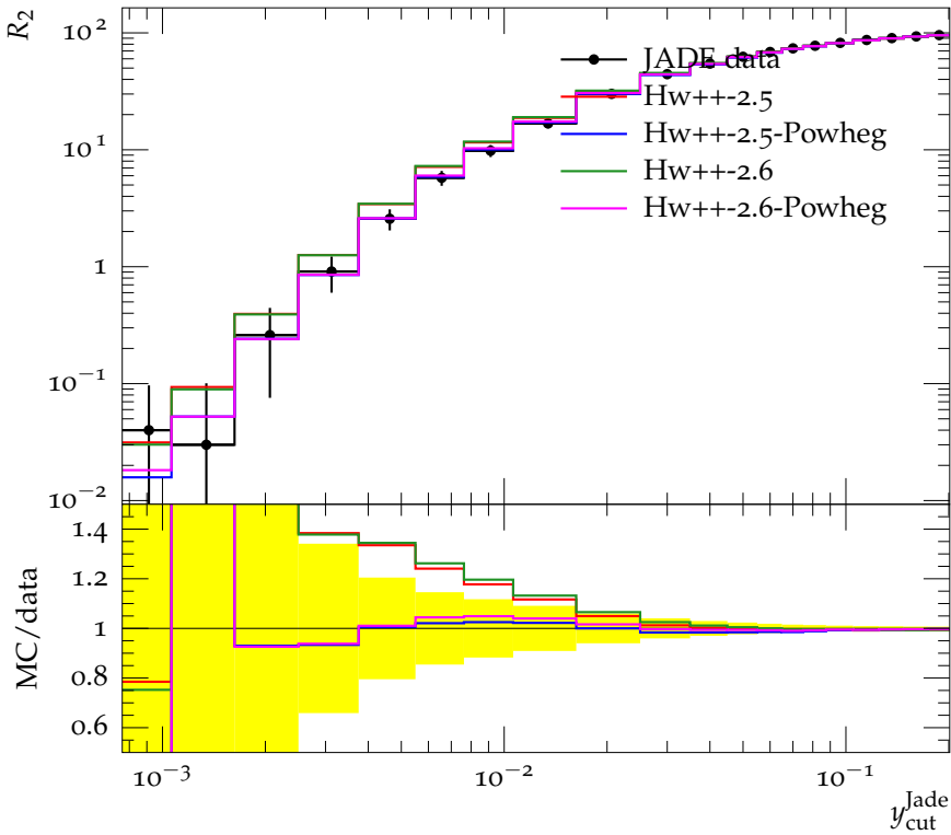
Integrated 2-jet rate with Jade algorithm (35 GeV)
