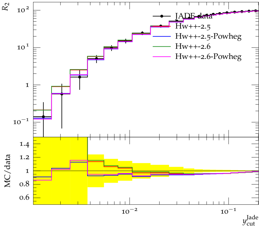
Integrated 2-jet rate with Jade algorithm (44 GeV)
