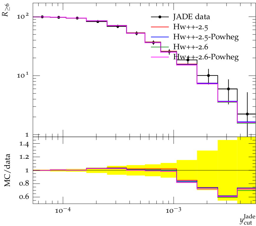
Integrated \geq 6 -jet rate with Jade algorithm (161 GeV)
