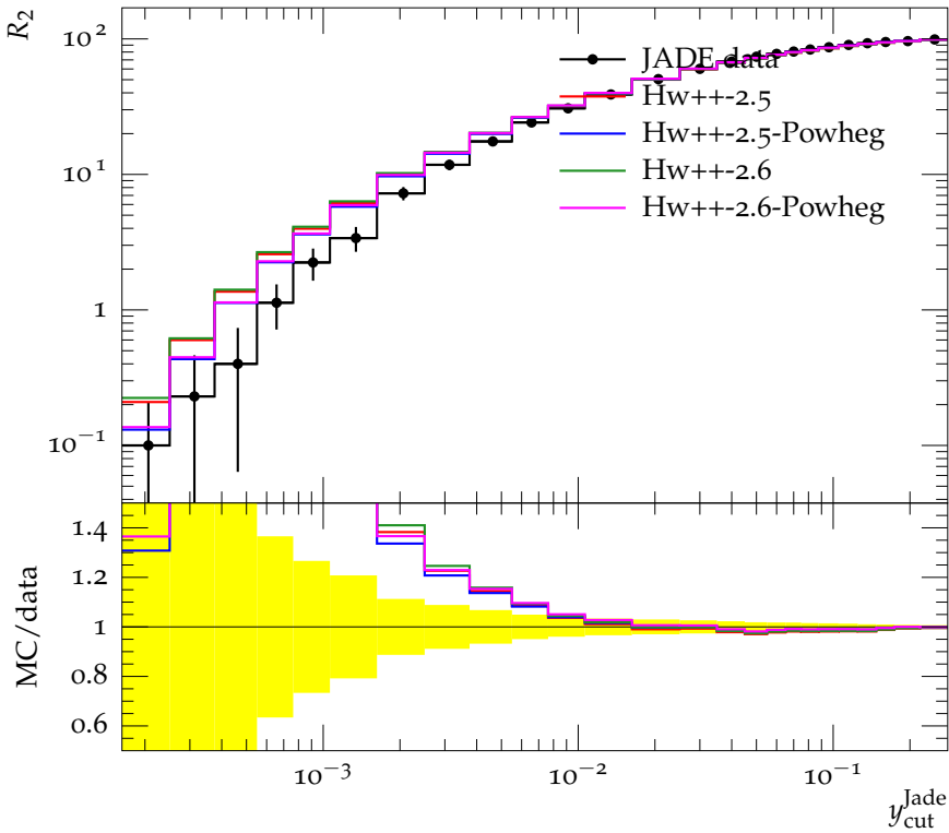
Integrated 2-jet rate with Jade algorithm (189 GeV)
