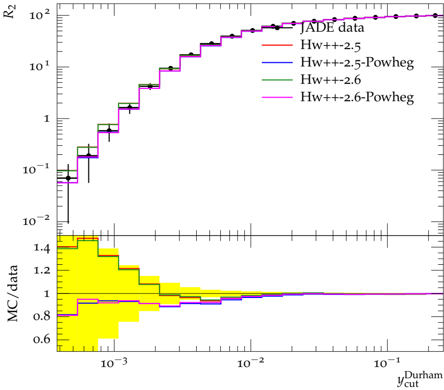
Integrated 2-jet rate with Durham algorithm (35 GeV)
