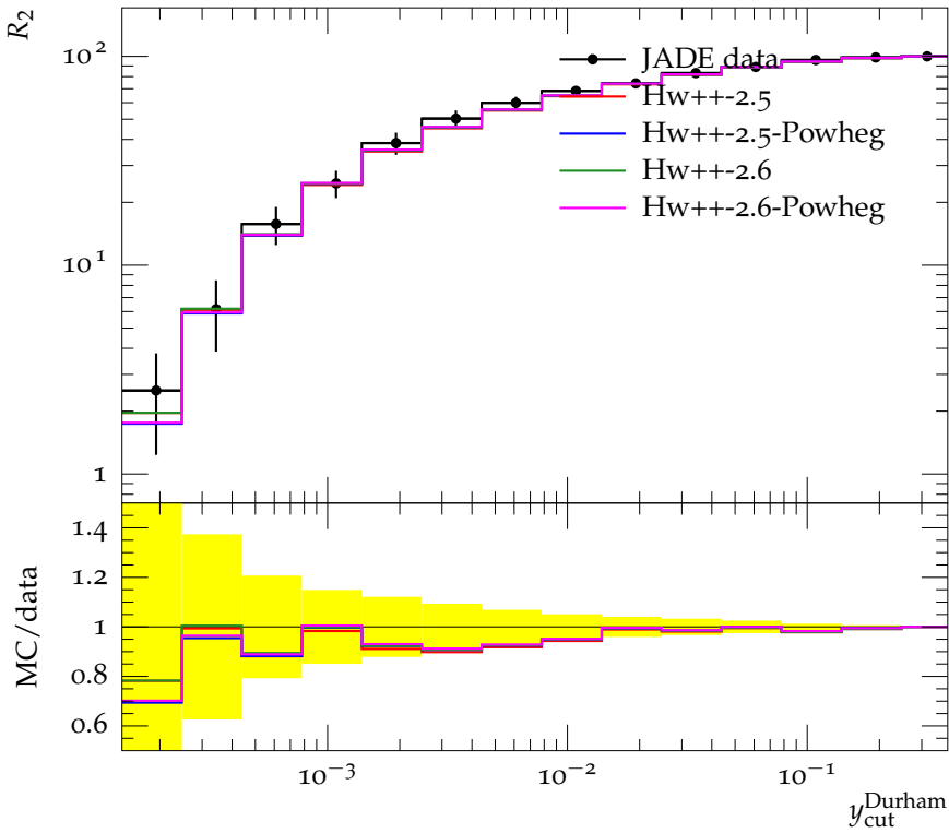
Integrated 2-jet rate with Durham algorithm (161 GeV)
