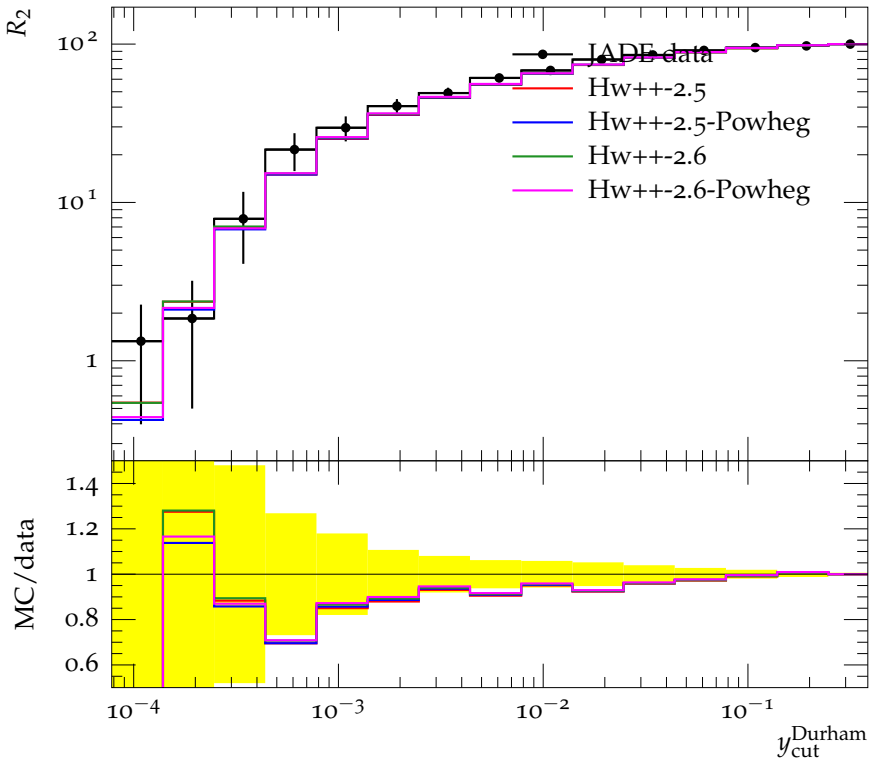
Integrated 2-jet rate with Durham algorithm (172 GeV)
