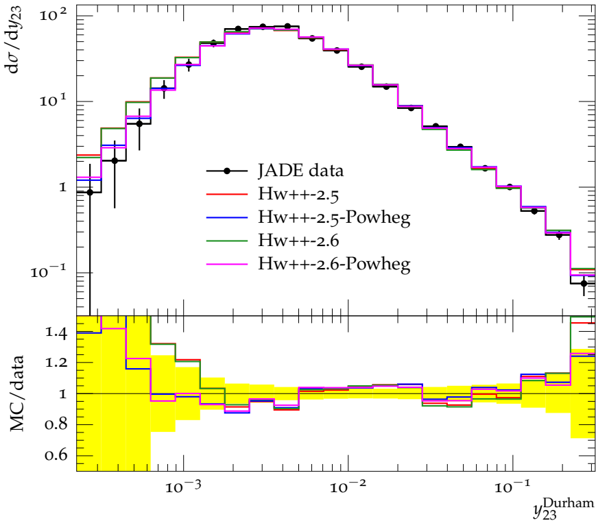
Differential 2-jet rate with Durham algorithm (35 GeV)
