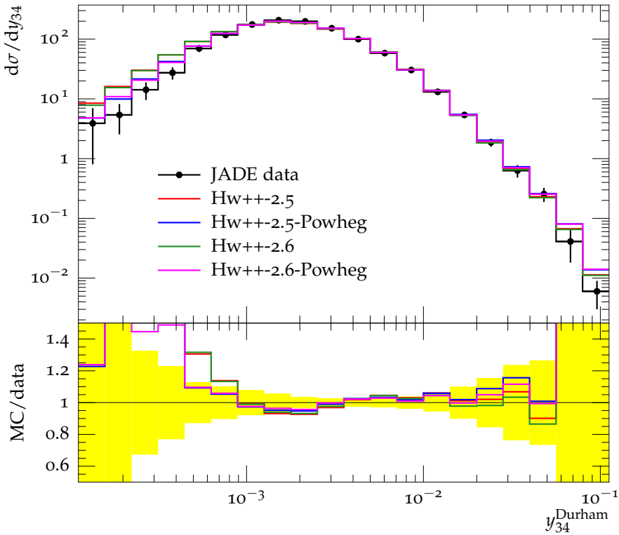
Differential 3-jet rate with Durham algorithm (35 GeV)
