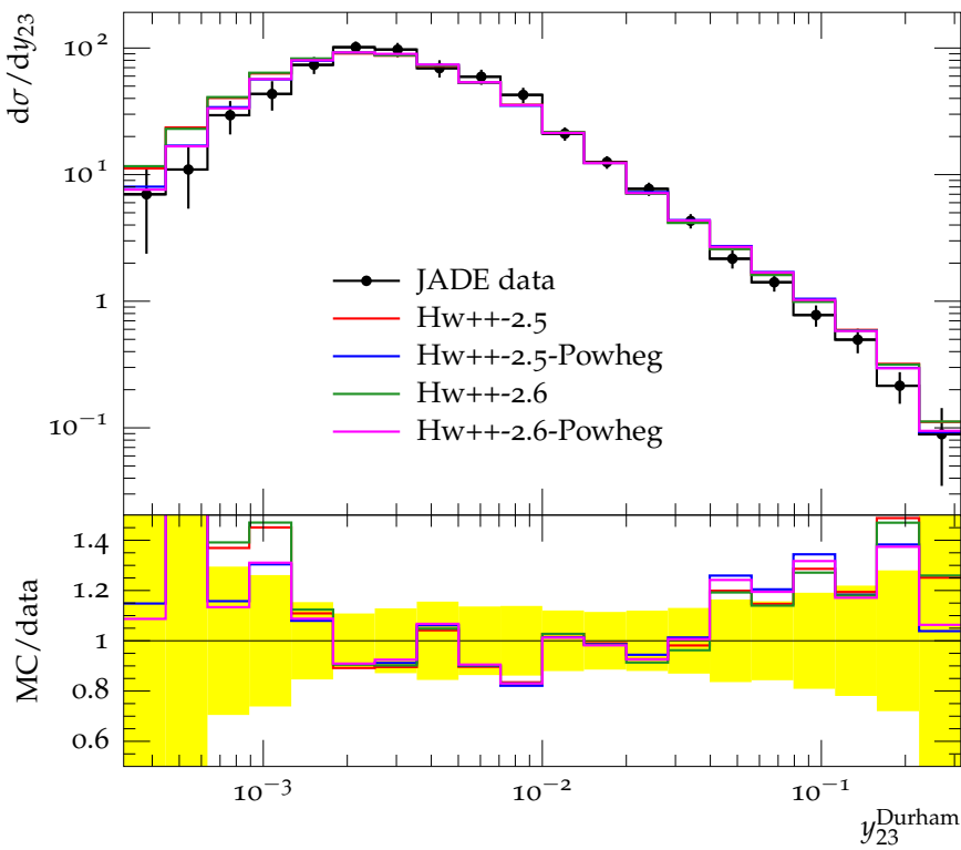
Differential 2-jet rate with Durham algorithm (44 GeV)
