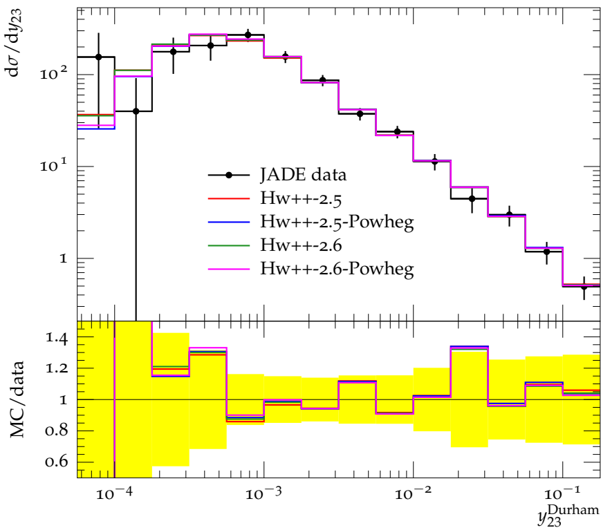
Differential 2-jet rate with Durham algorithm (133 GeV)
