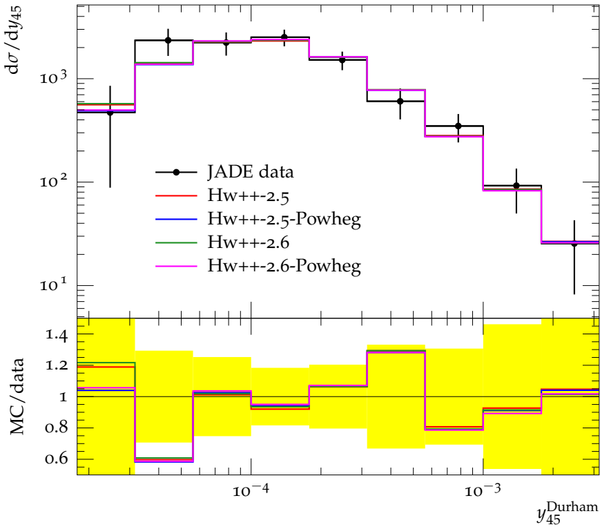
Differential 4-jet rate with Durham algorithm (172 GeV)
