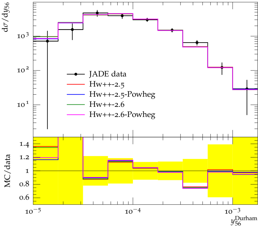
Differential 5-jet rate with Durham algorithm (183 GeV)
