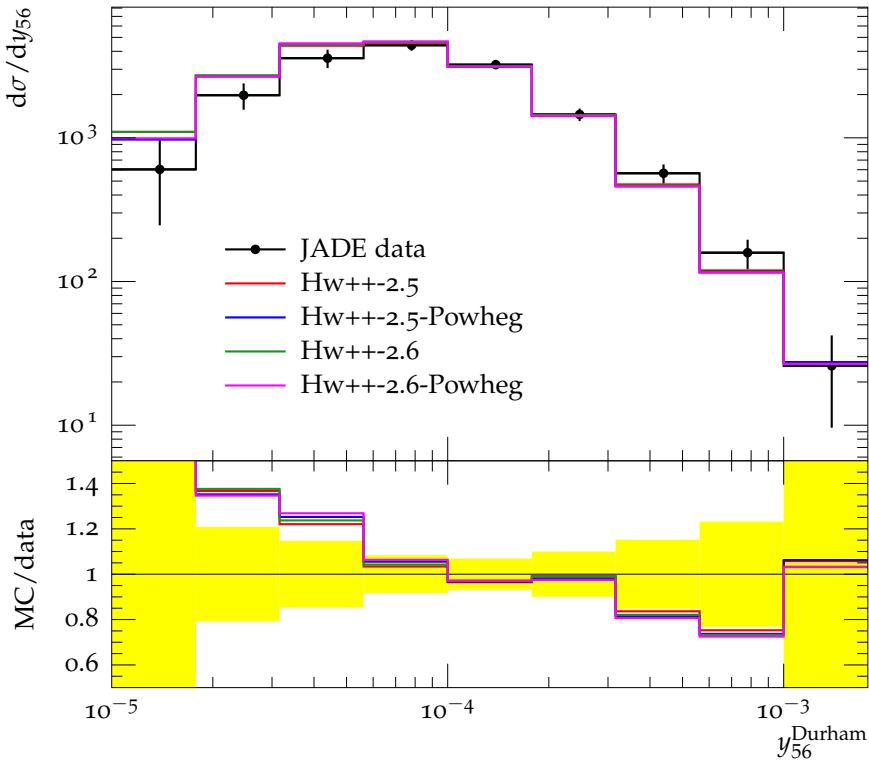
Differential 5-jet rate with Durham algorithm (189 GeV)
