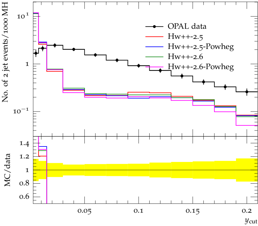
Number of 2 jet events vs y_{cut} , Jade
