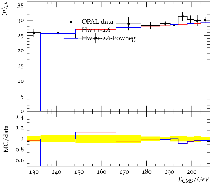
Charged multiplicity as a function of energy in b events
