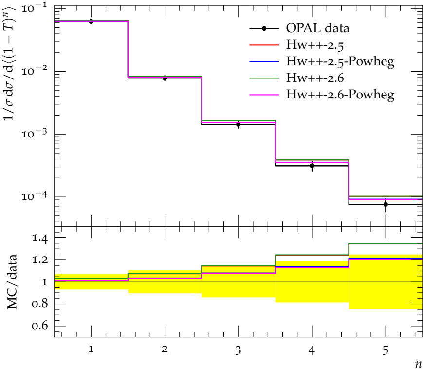
Moments of 1 - T at 133 GeV
