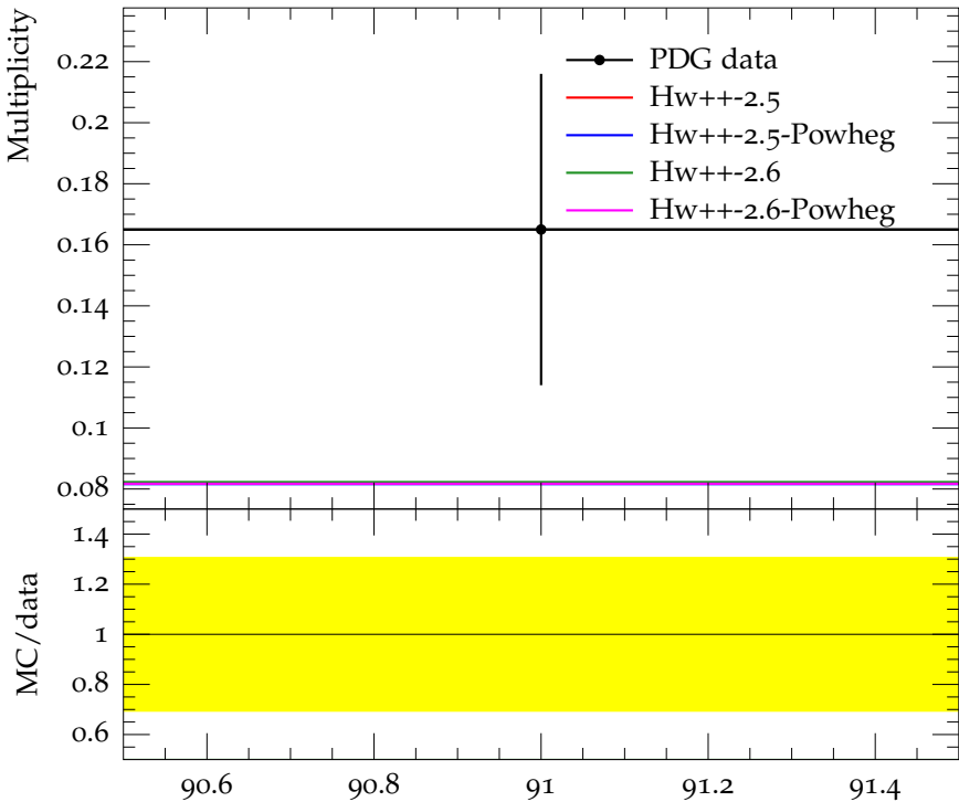
Mean f_1(1285) multiplicity
