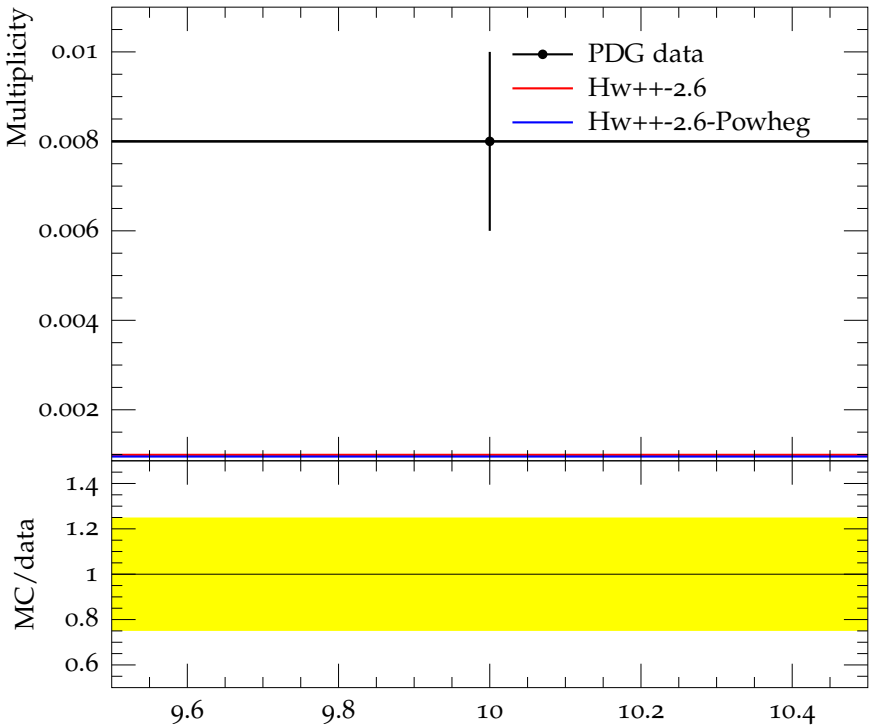
Mean \Lambda(1520) multiplicity
