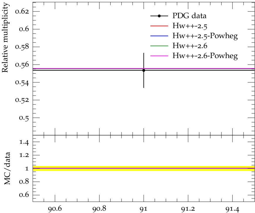
Ratio (w.r.t. \pi^\pm ) of mean \pi^0 multiplicity
