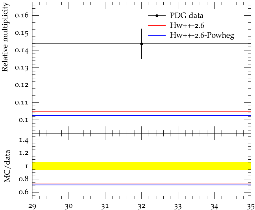
Ratio (w.r.t. \pi^\pm ) of mean K^0 multiplicity
