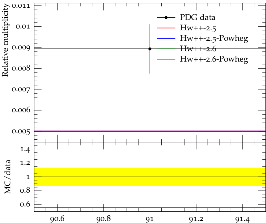
Ratio (w.r.t. \pi^\pm ) of mean \eta'(958) multiplicity
