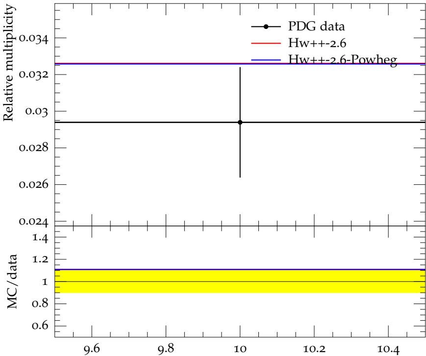
Ratio (w.r.t. \pi^\pm ) of mean D^+ multiplicity
