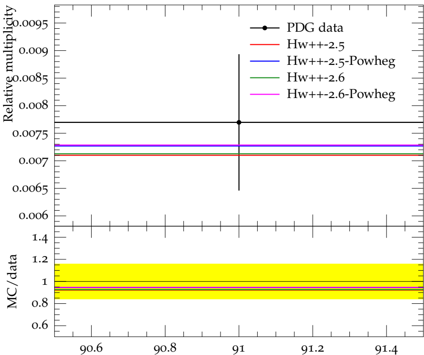
Ratio (w.r.t. \pi^\pm ) of mean D_s^+ multiplicity
