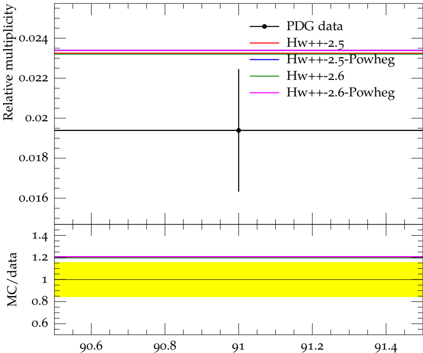
Ratio (w.r.t. \pi^\pm ) of mean B^+, B_d^0 multiplicity
