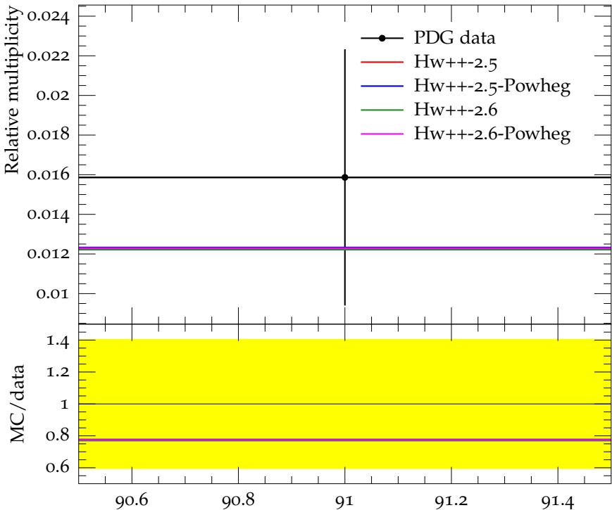
Ratio (w.r.t. \pi^\pm ) of mean a_0^+ (980) multiplicity
