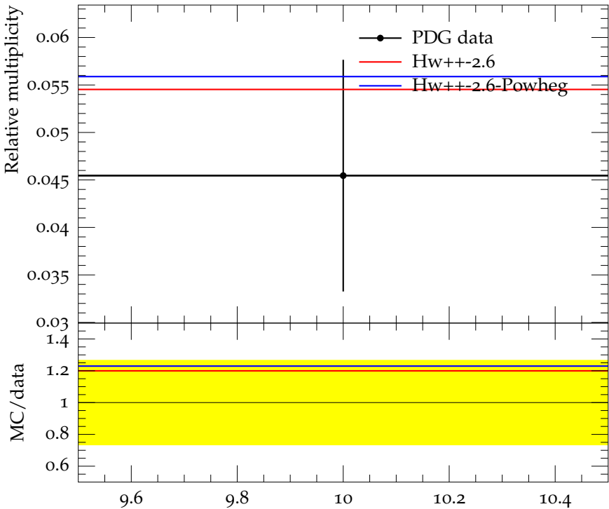
Ratio (w.r.t. \pi^\pm ) of mean \omega(782) multiplicity
