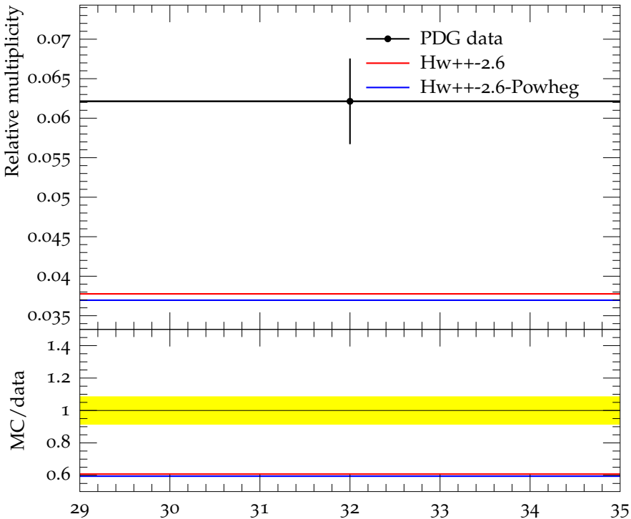
Ratio (w.r.t. \pi^\pm ) of mean K^{*+}(892) multiplicity
