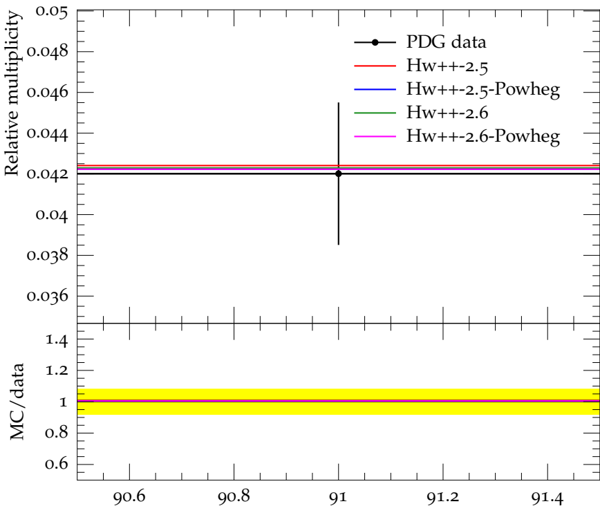
Ratio (w.r.t. \pi^\pm ) of mean K^{*+} (892) multiplicity
