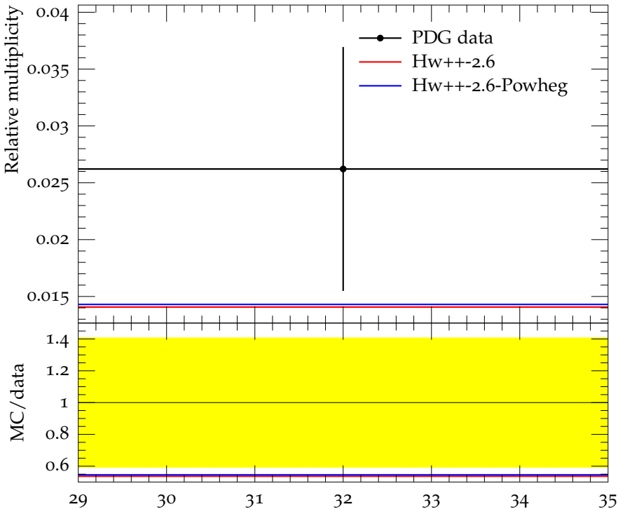
Ratio (w.r.t. \pi^\pm ) of mean D^{*0} (2007) multiplicity
