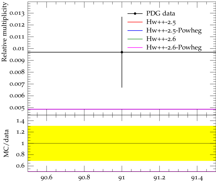
Ratio (w.r.t. \pi^\pm ) of mean f_1(1285) multiplicity
