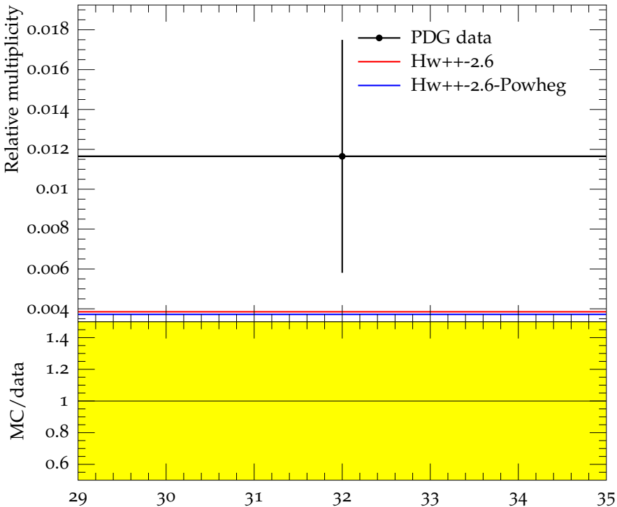
Ratio (w.r.t. \pi^\pm ) of mean K_2^{*0}(1430) multiplicity
