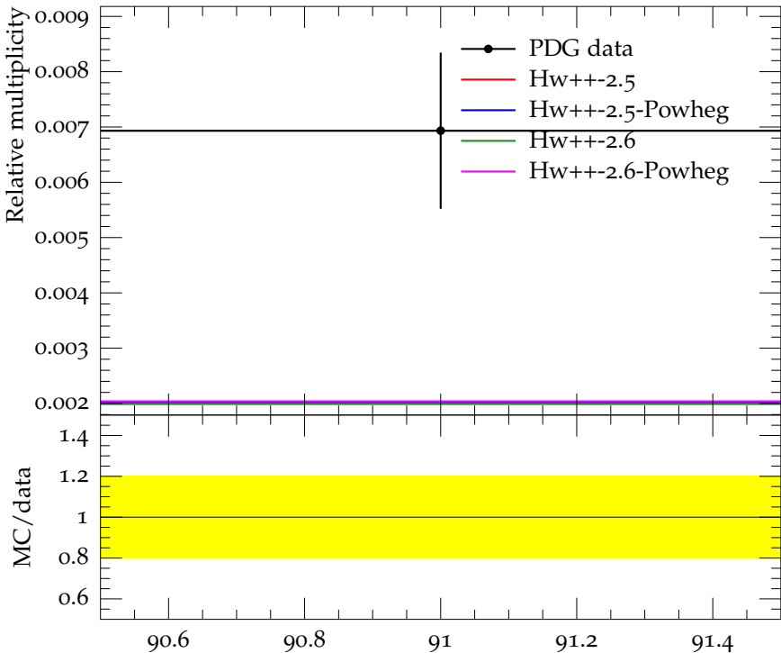
Ratio (w.r.t. \pi^\pm ) of mean B^{**} multiplicity
