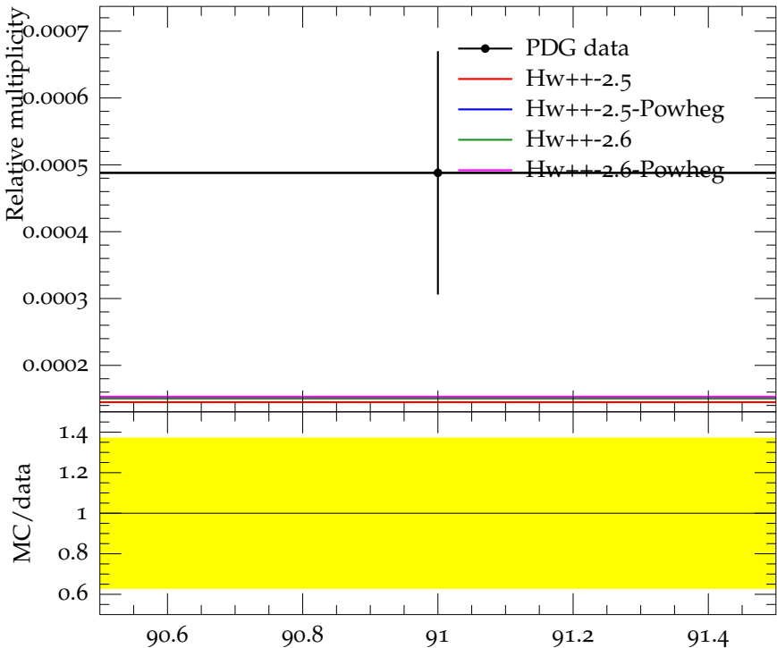
Ratio (w.r.t. \pi^\pm ) of mean D_{s2}^+ multiplicity
